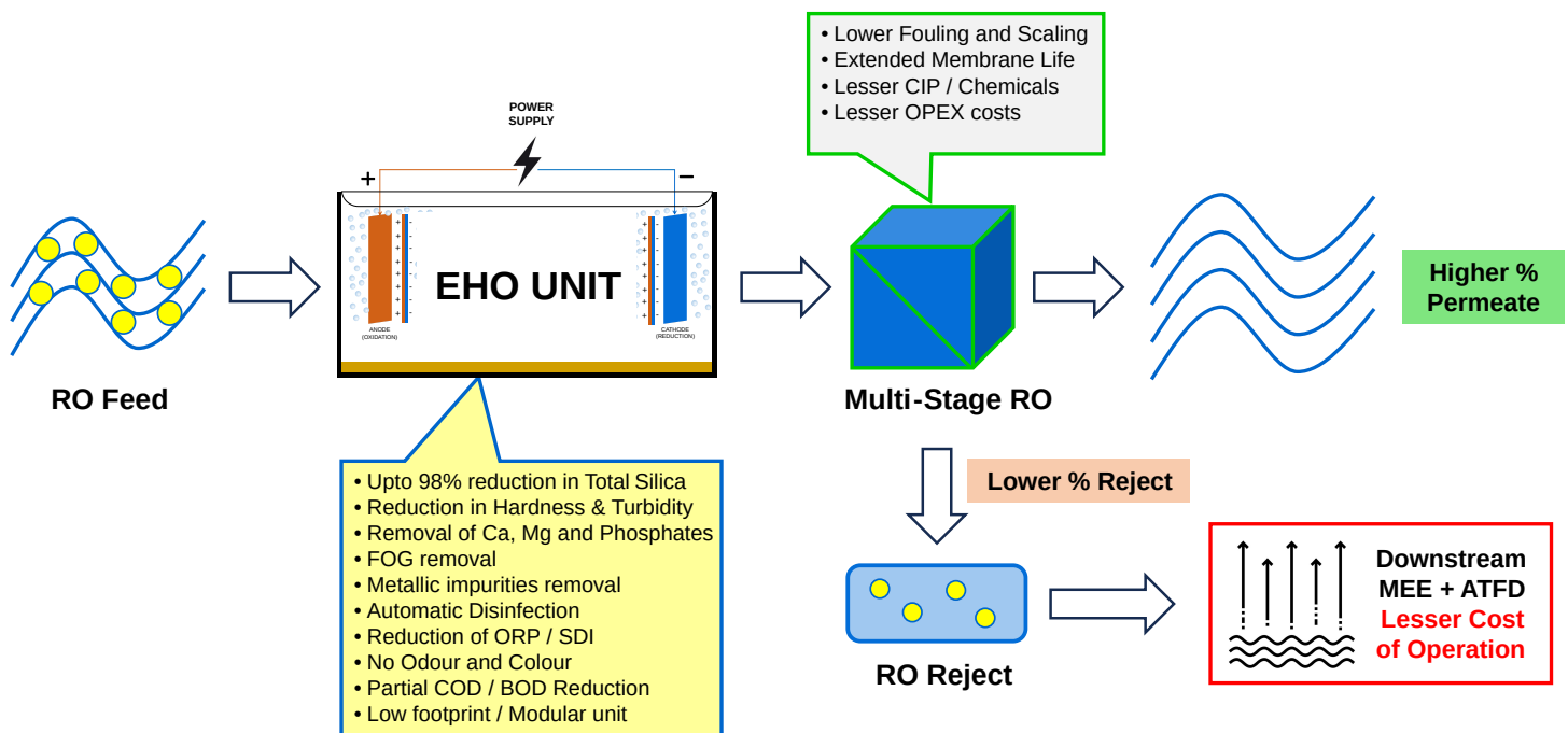
Typical installation schematic of the Boson Alchemies EHO unit; The unit can also be installed in between RO stages for higher permeate recovery
